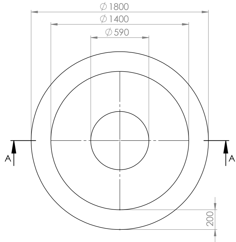
Top View
